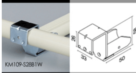
[ SLIDE PIPE METAL-B1 ]
