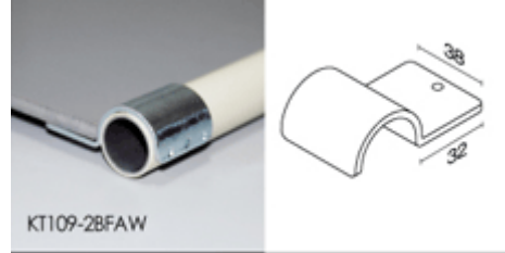
[ BOARD FIXING METAL-A ]
