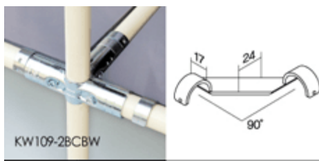
[ BOARD FIXING CORNER METAL-B ]
