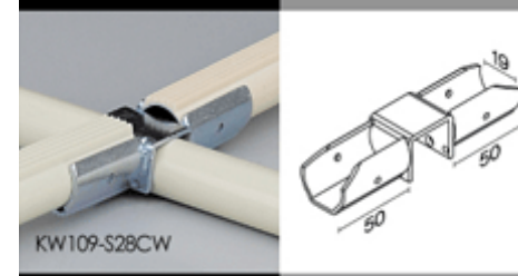
[ SLIDE PIPE METAL-C ]
