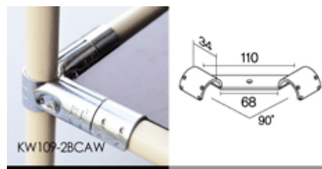
[ BOARD FIXING CORNER METAL-A ]
